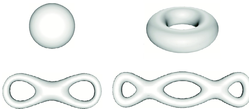
Figure 10. Domains of various topological types.
