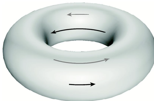
Figure 6. A vector field in the subspace HK of harmonic knots.
