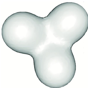
Figure 11. A domain homeomorphic to a ball.
