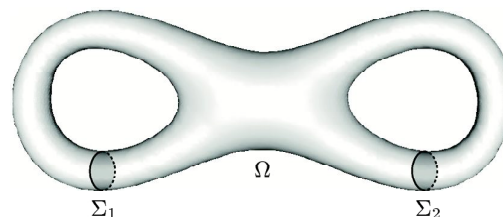
Figure 2. A domain with cross-sectional disks.
