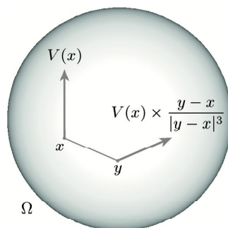
Figure 8. The Biot-Savart integrand.
